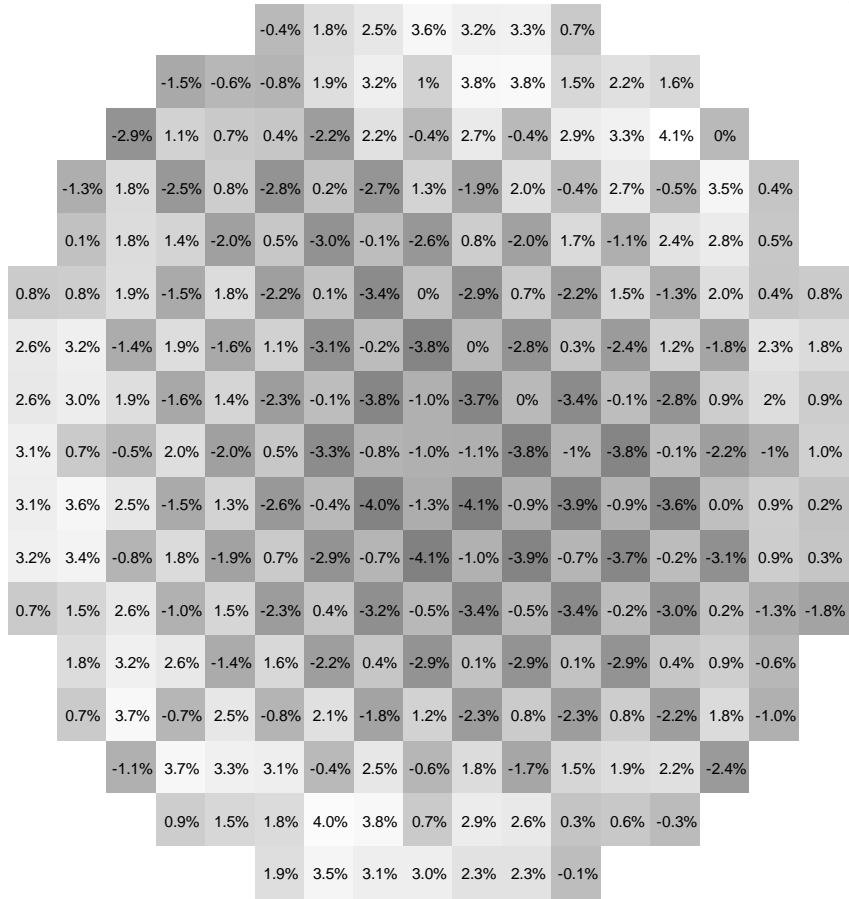
Figure 12 - Power distribution of the perturbed UOX core: relative differences between QUABOX/CUBBOX and KENO V.a
