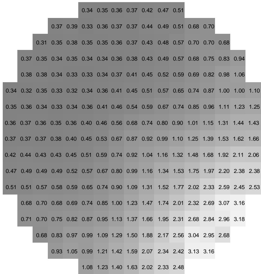
Figure 11 - KENO V.a power distribution of the pertured UOX core
