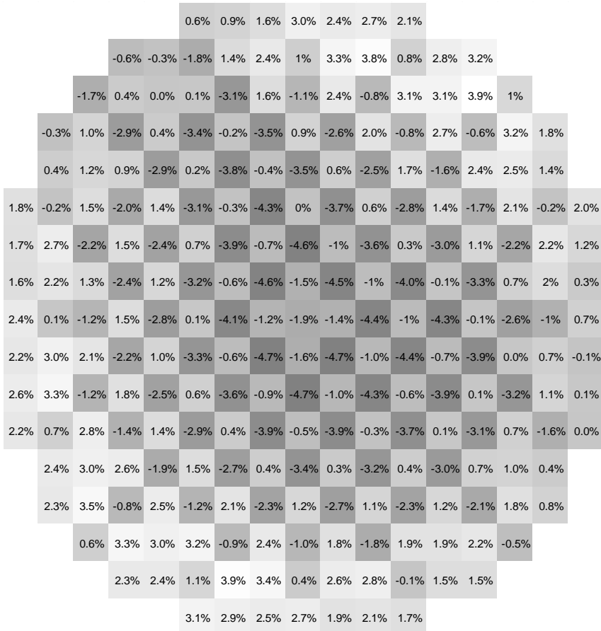
Figure 13 - Power distribution of the perturbed UOX core: relative differences between PARCS and KENO V.a
