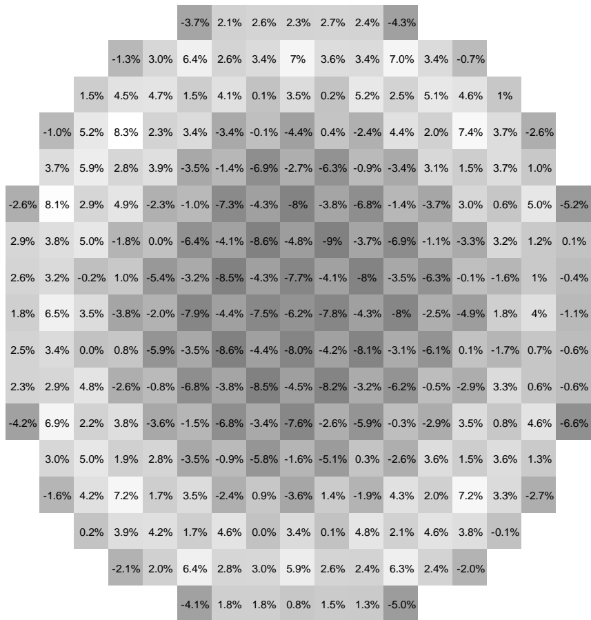
Figure 14 - Power distribution of the perturbed UOX core: relative differences between DONJON and KENO V.a
